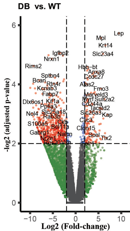
Supplementary Fig. 2. Volcano plot suggesting the differentially expressed genes (DEGs) from cardiac RNA sequencing public data between db/db or C57BLKS/J (BKS) mice. The threshold of the y-axis is the cutoff of the adjusted \log_2 ( P value), which is 2. WT, wild type.
