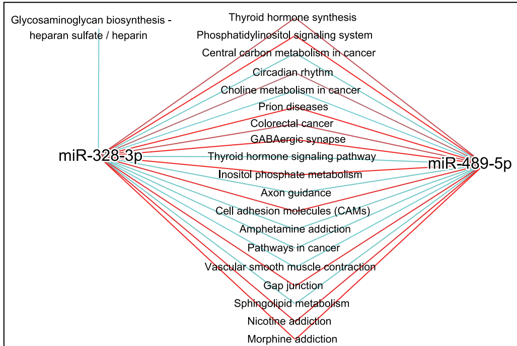
Supplementary Fig. 3. Kyoto Encyclopedia of Genes and Genomes (KEGG) enrichment analysis of highly expressed and conserved miRNA target genes using the mirPATH tool in the DIANA database.
