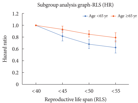
Supplementary Fig. 1. Subgroup analysis for hazard ratios (HRs) of severe hypoglycemia by reproductive life span for subgroup aged <65, and \geq 65 in postmenopausal women with type 2 diabetes mellitus. The inverse association of reproductive life span (RLS) with severe hypoglycemia (SH) risk was more evident in women below 65 years.
