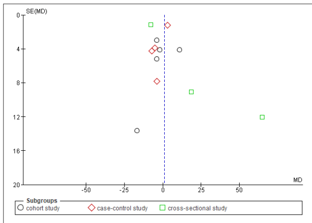
Supplementary Fig. 2. Funnel plot for 12 studies of random blood glucose. SE, standard error; MD, mean difference.
