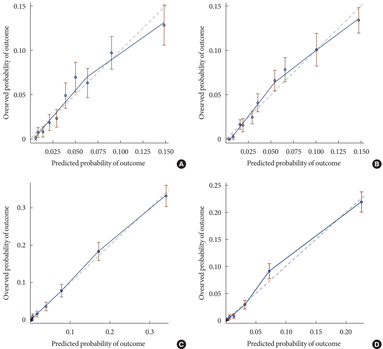
Supplementary Fig. 2. Calibration plot: diabetes mellitus (A, United States & B, Korea) & chronic kidney disease (C, United States & D, Korea).
