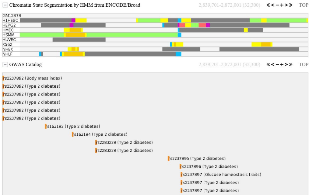
Supplementary Fig. 4. Previous genome-wide association study (GWAS) results in potassium voltage-gated channel subfamily Q member 1 ( KCNQ1 ) gene region. As shown, in the KCNQ1 gene region, there are many genome-wide significant loci for type 2 diabetes mellitus development. HMM, hidden Markov model.
