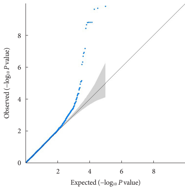
Supplementary Fig. 1. Quantile-quantile plot of P values from genome-wide association study.
